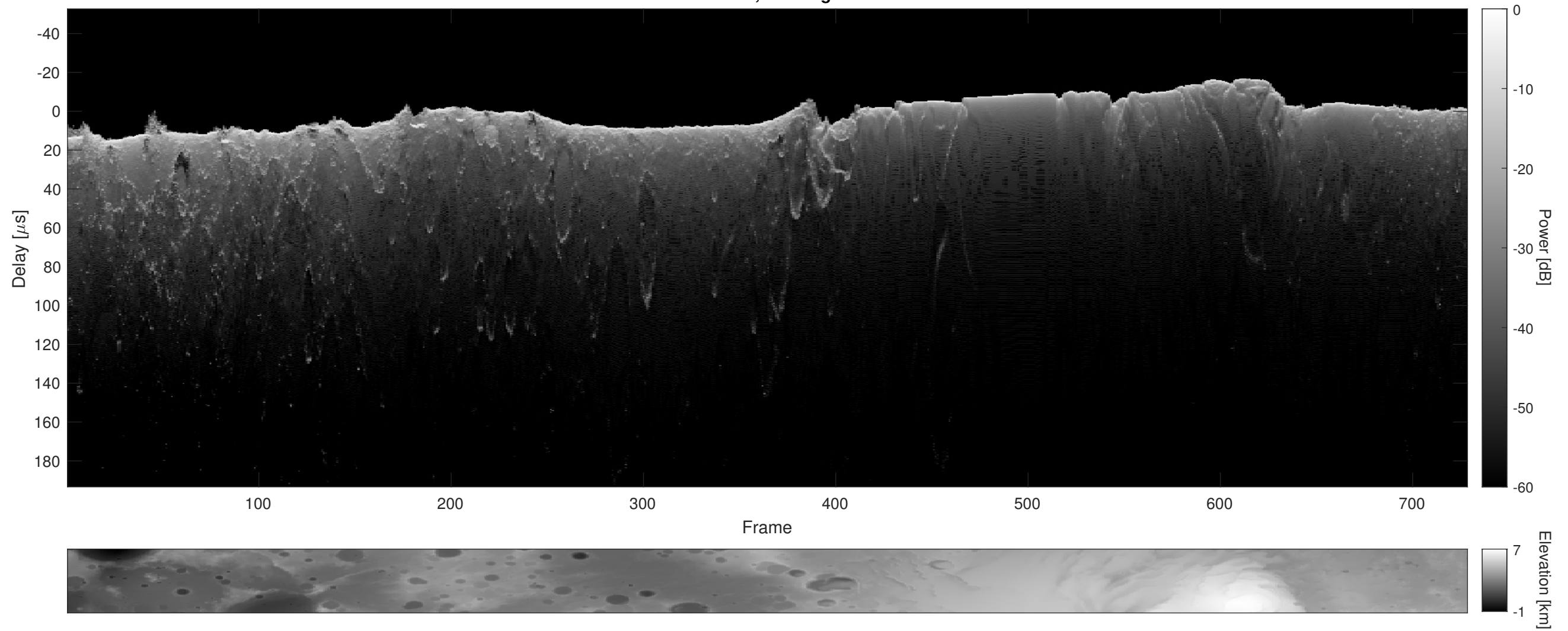
Orbit 4588, Cluttergram
