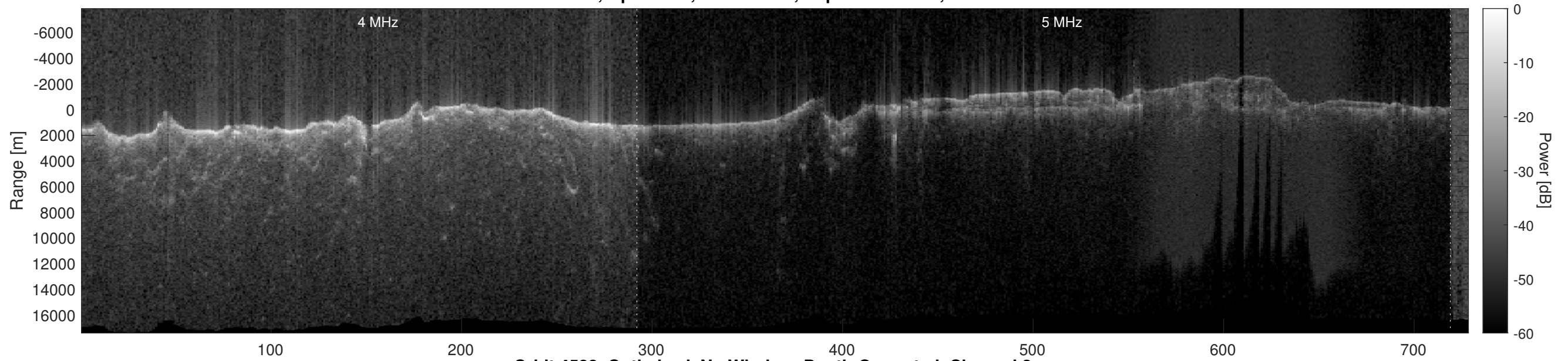
Orbit 4588, Optimized, No Window, Depth-Corrected, Channel 2
