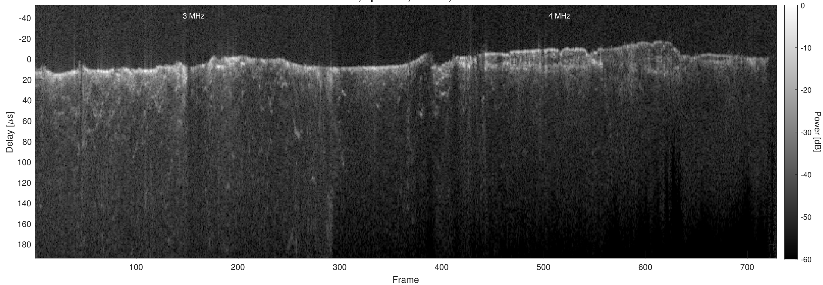
Orbit 4588, Optimized, Window, Channel 2
