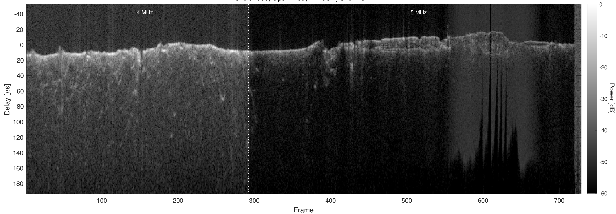
Orbit 4588, Optimized, Window, Channel 2
