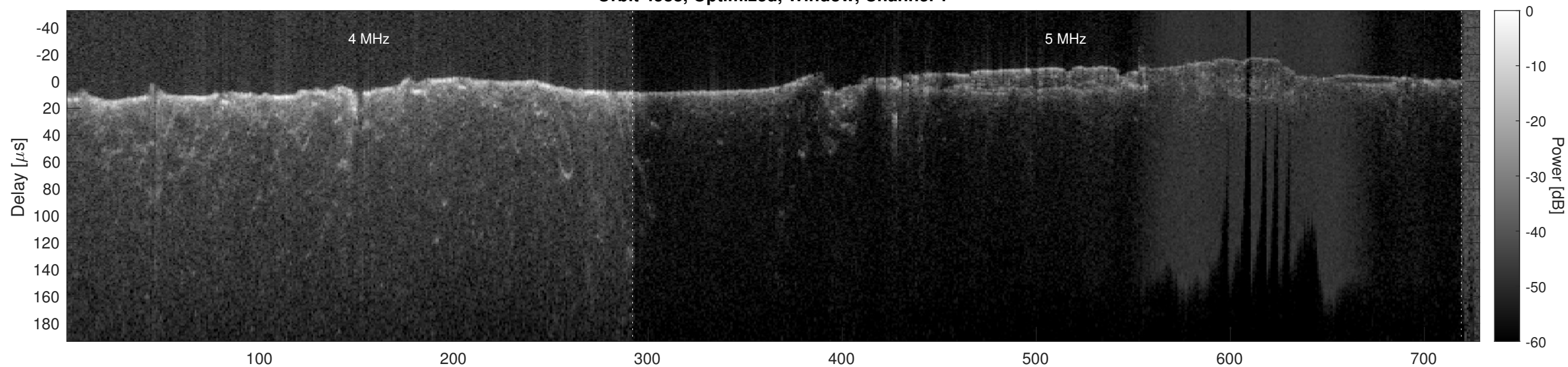
Orbit 4588, Optimized, Window, Channel 2
