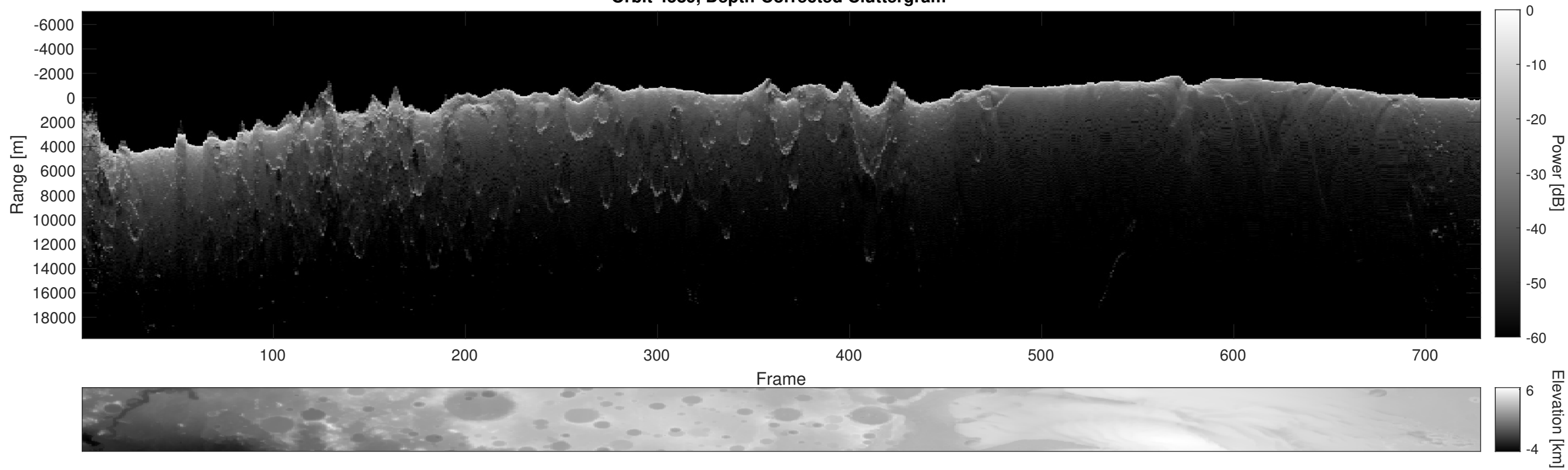
Orbit 4589, Depth-Corrected Cluttergram
