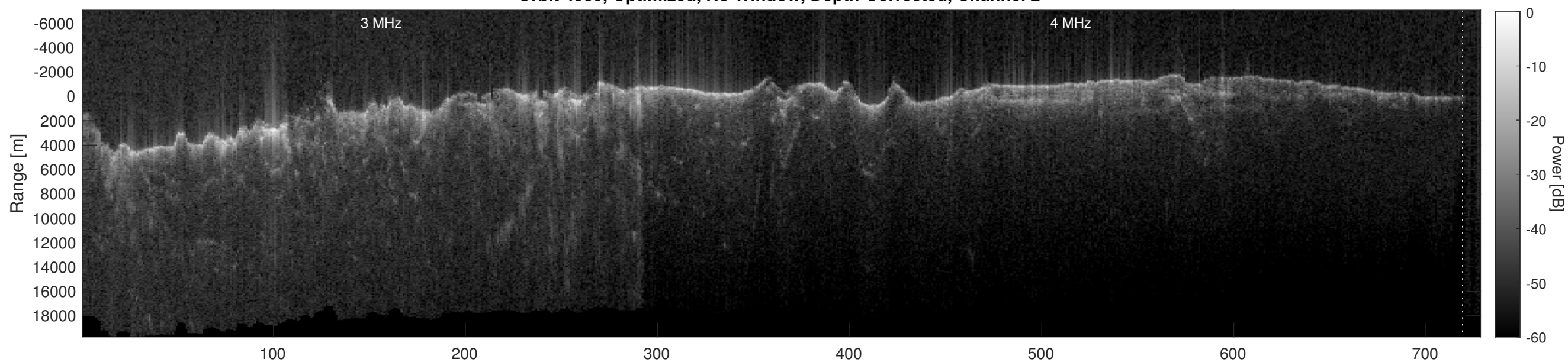
Orbit 4589, Depth-Corrected Cluttergram
