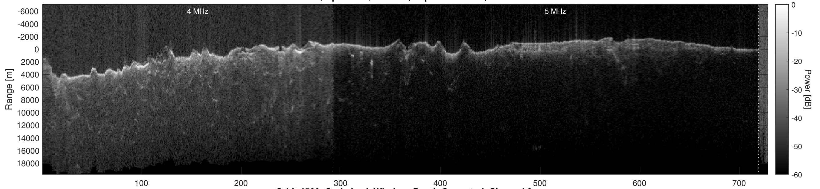
Orbit 4589, Optimized, Window, Depth-Corrected, Channel 2
