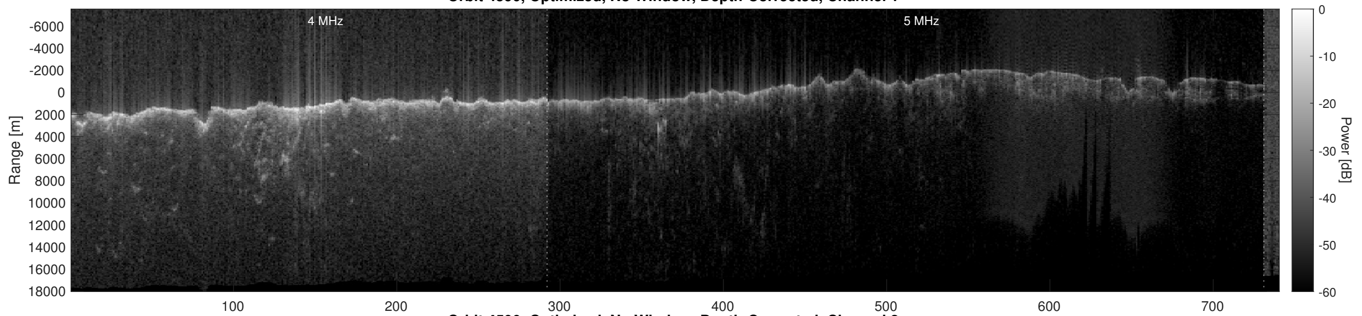
Orbit 4590, Optimized, No Window, Depth-Corrected, Channel 2
