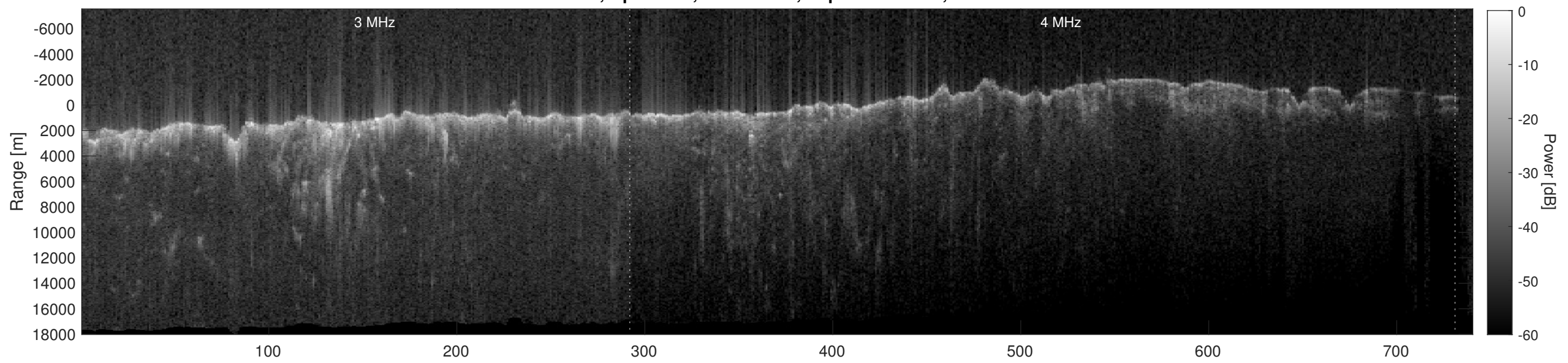
Orbit 4590, Depth-Corrected Cluttergram
