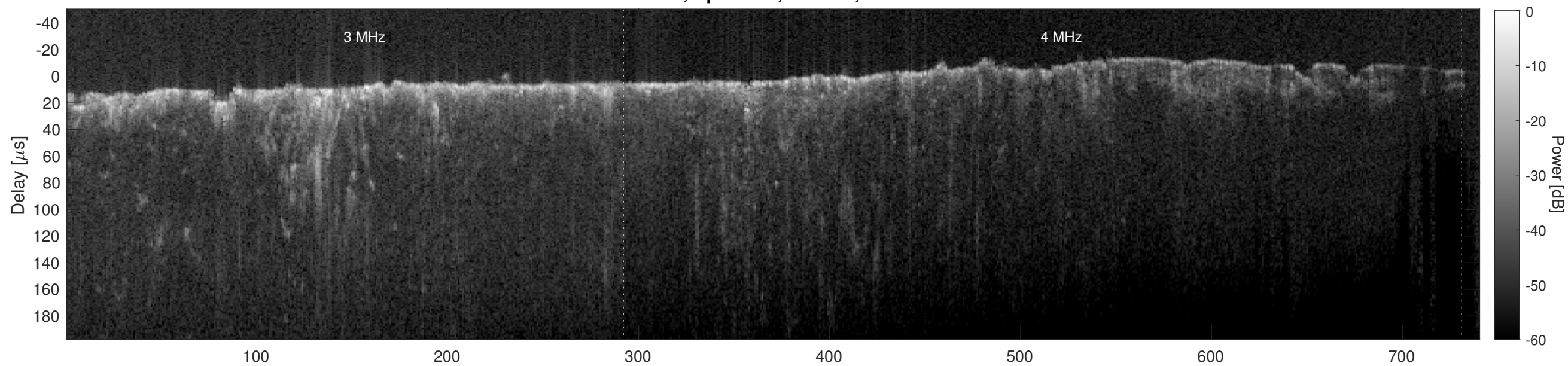
Orbit 4590, Cluttergram
