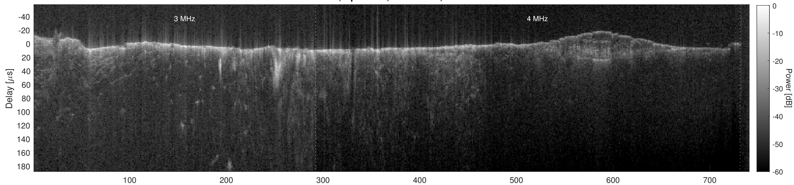
Orbit 4591, Cluttergram
