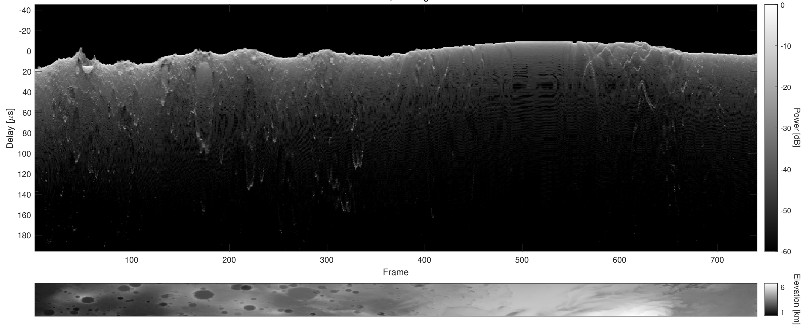
Orbit 4592, Cluttergram
