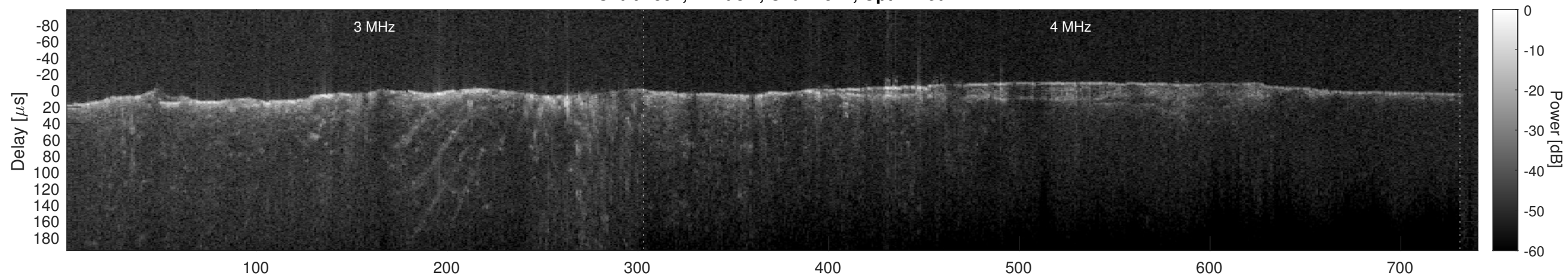
Orbit 4592, Cluttergram
