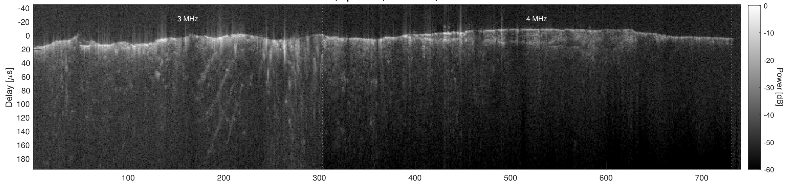
Orbit 4592, Cluttergram
