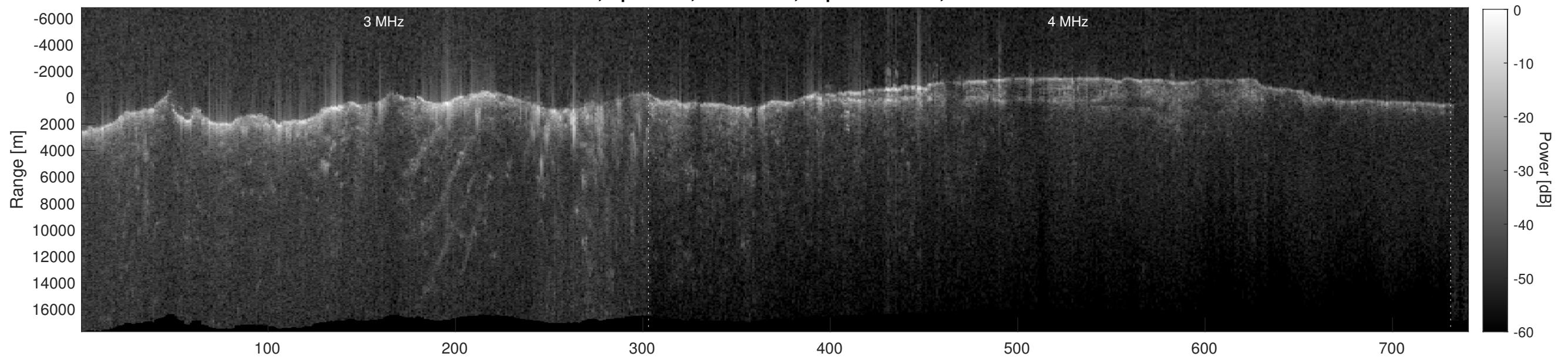
Orbit 4592, Depth-Corrected Cluttergram
