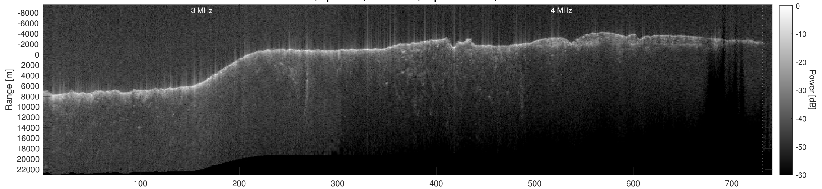
Orbit 4593, Depth-Corrected Cluttergram
