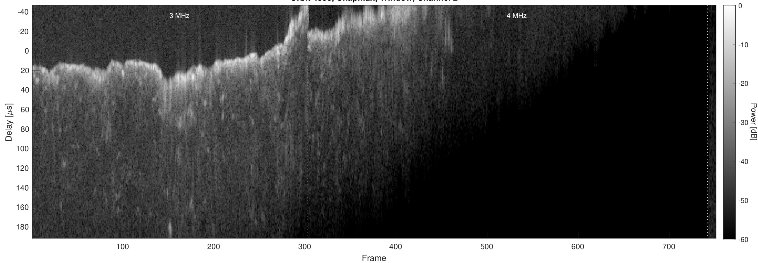
Orbit 4596, Chapman, Window, Channel 2
