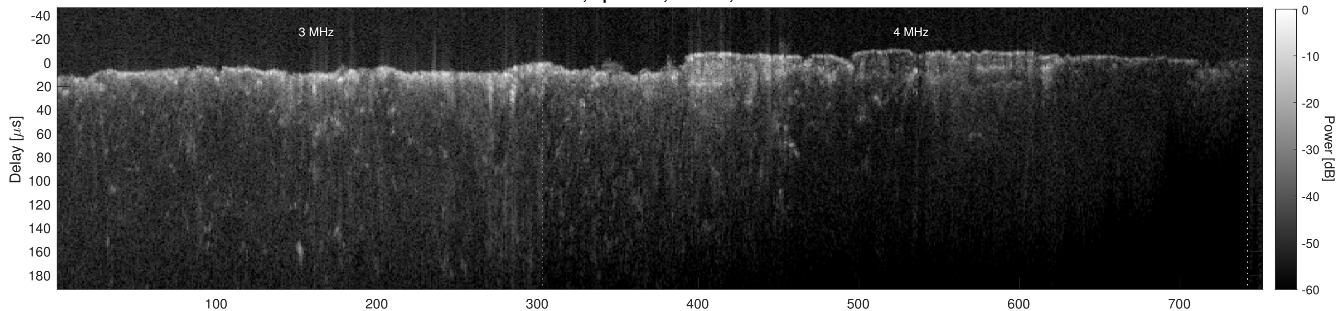
Orbit 4596, Cluttergram
