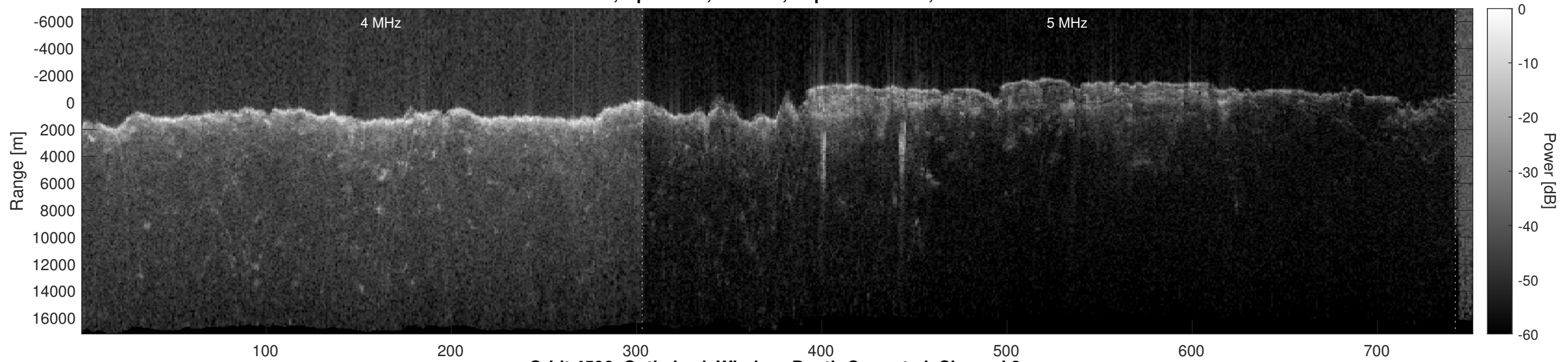
Orbit 4596, Optimized, Window, Depth-Corrected, Channel 2
