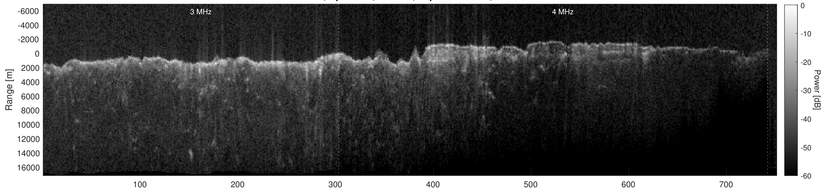
Orbit 4596, Depth-Corrected Cluttergram
