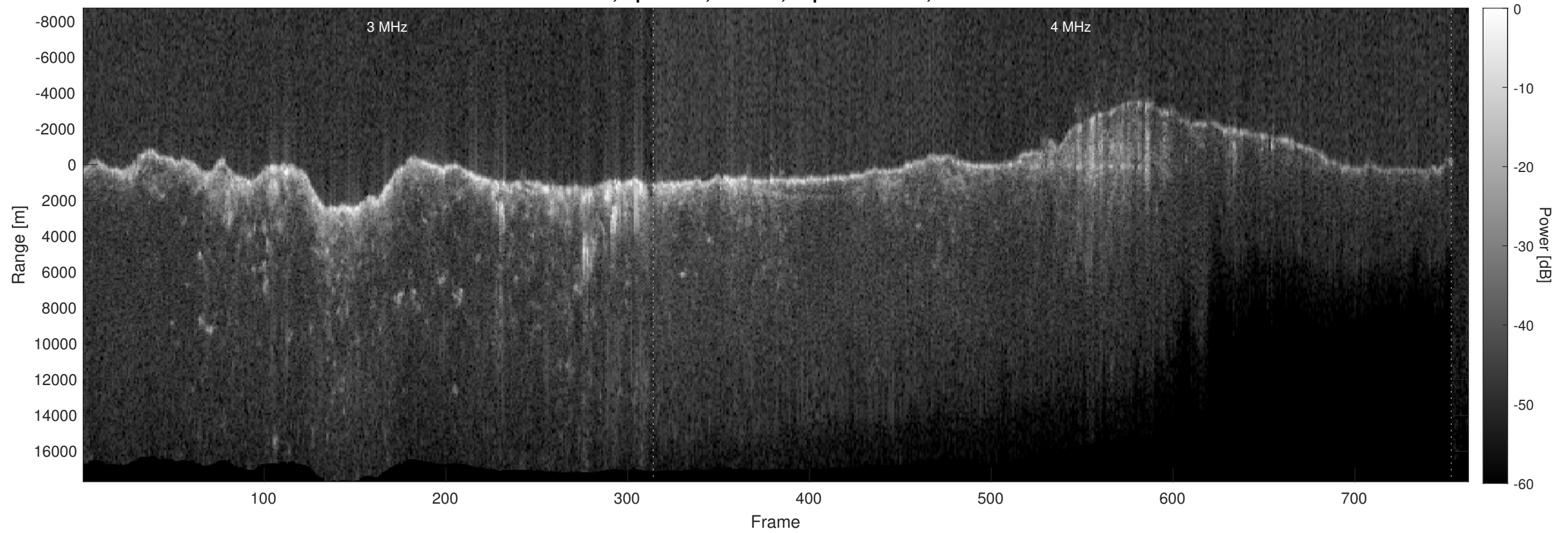
Orbit 4598, Optimized, Window, Depth-Corrected, Channel 2
