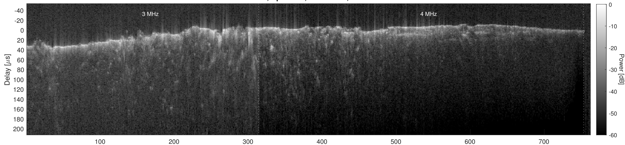
Orbit 4600, Cluttergram
