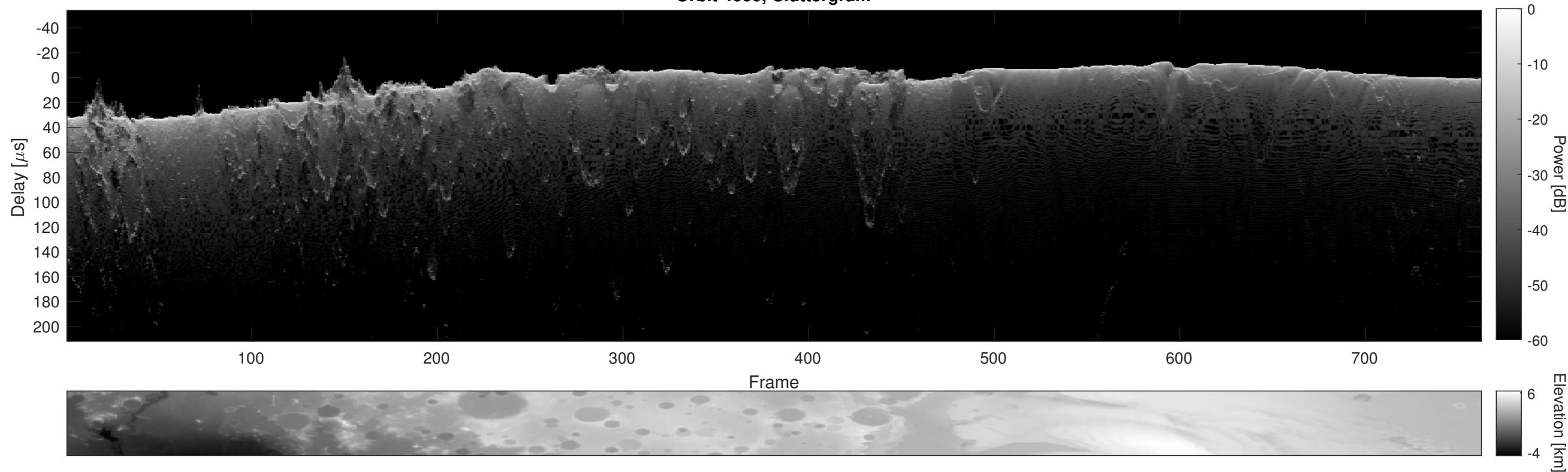
Orbit 4600, Cluttergram
