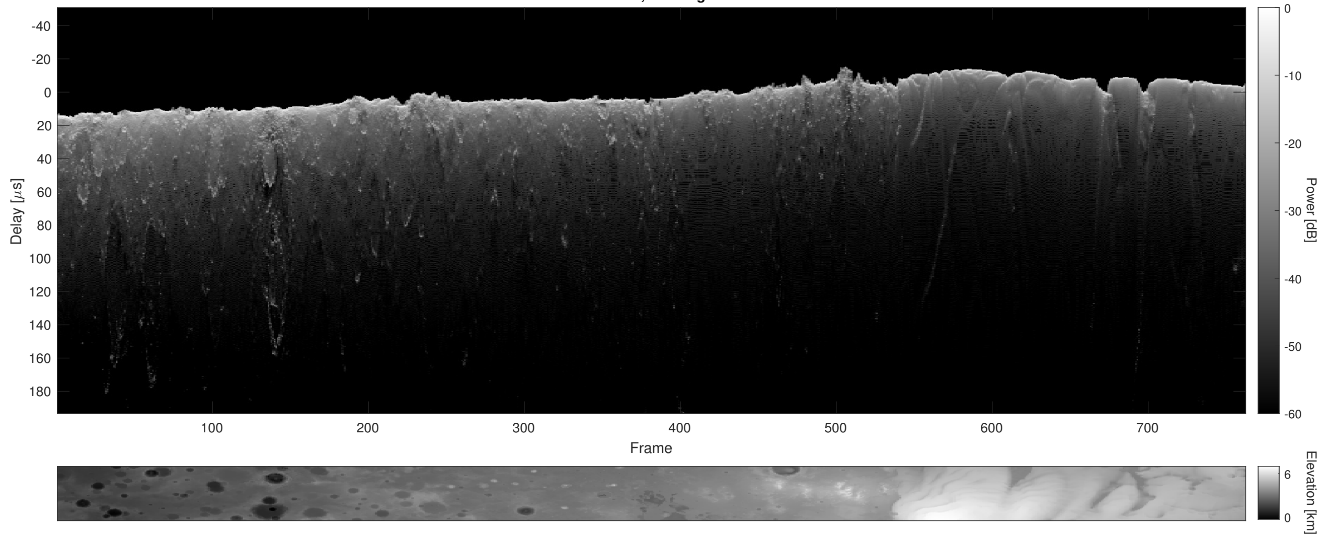
Orbit 4601, Cluttergram
