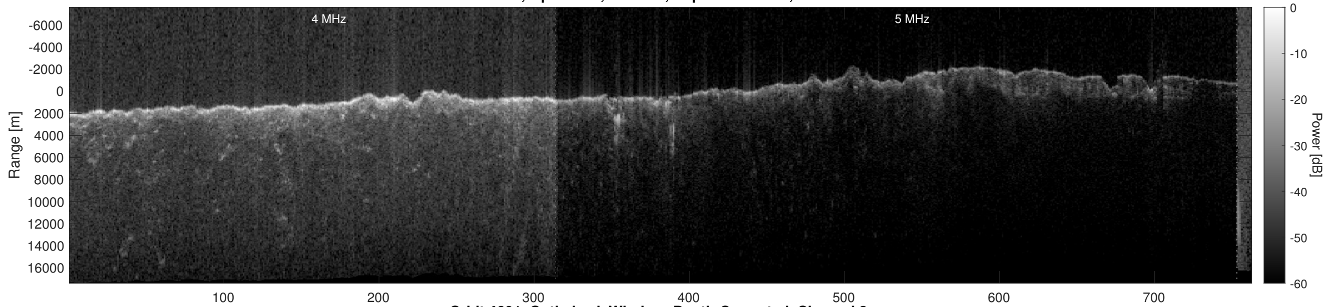
Orbit 4601, Optimized, Window, Depth-Corrected, Channel 2
