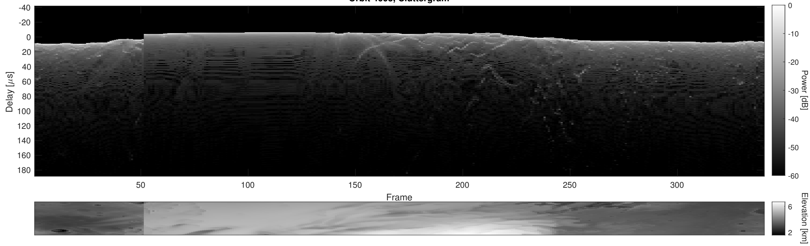
Orbit 4603, Cluttergram
