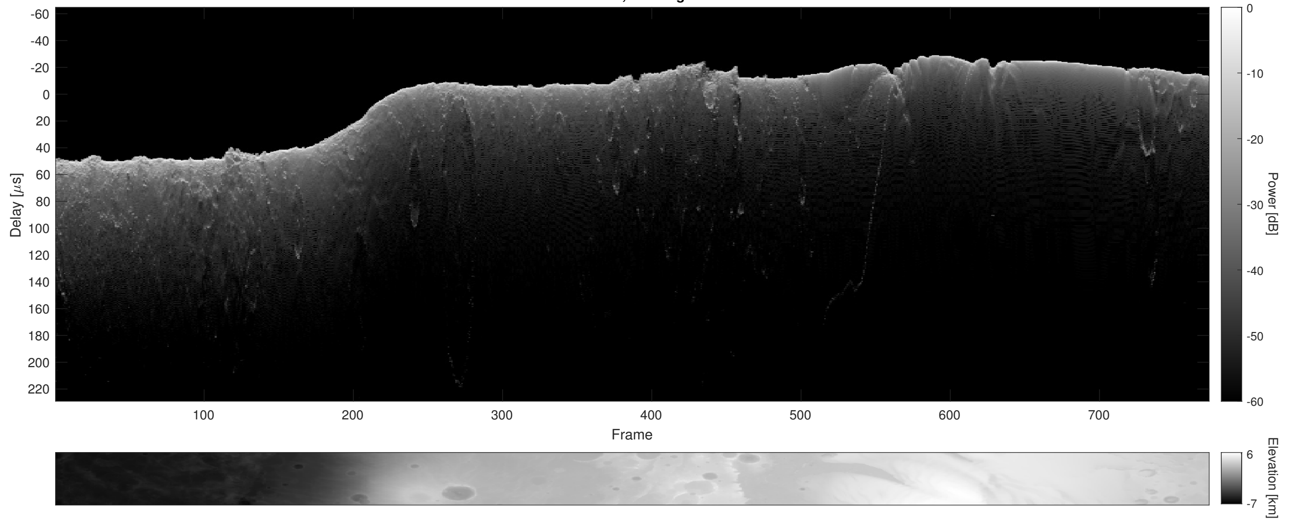
Orbit 4604, Cluttergram
