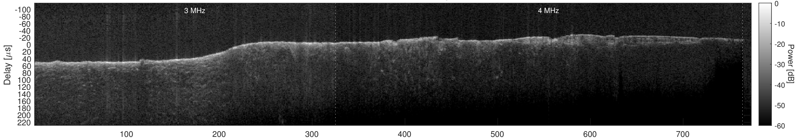
Orbit 4604, Cluttergram
