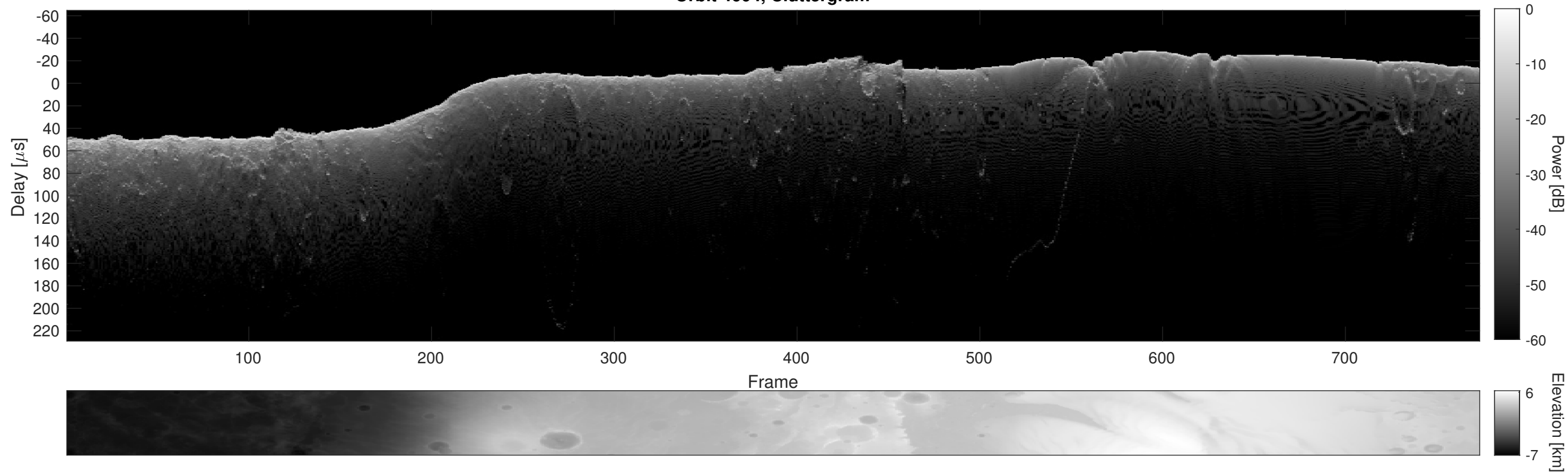
Orbit 4604, Cluttergram
