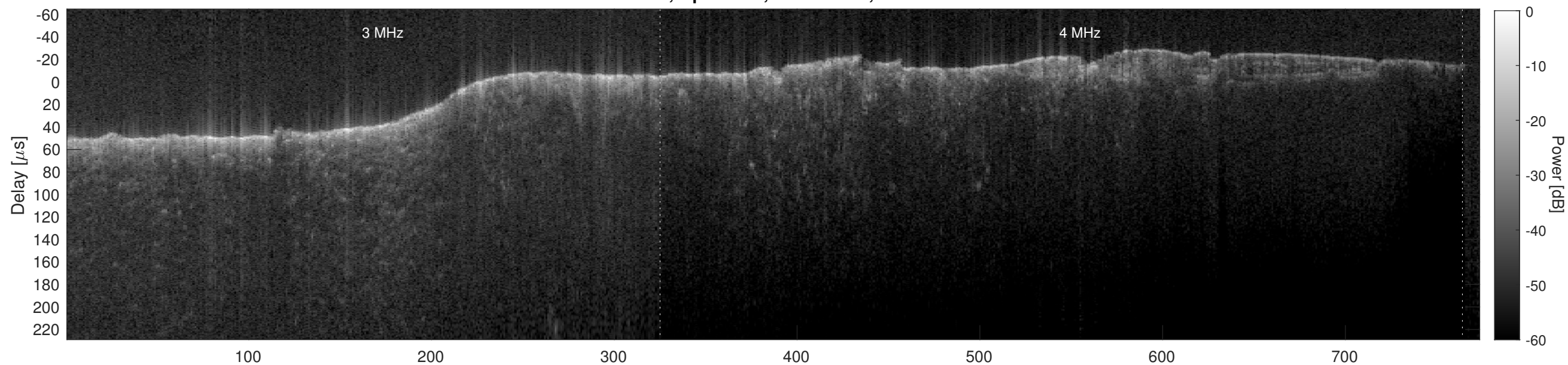
Orbit 4604, Cluttergram
