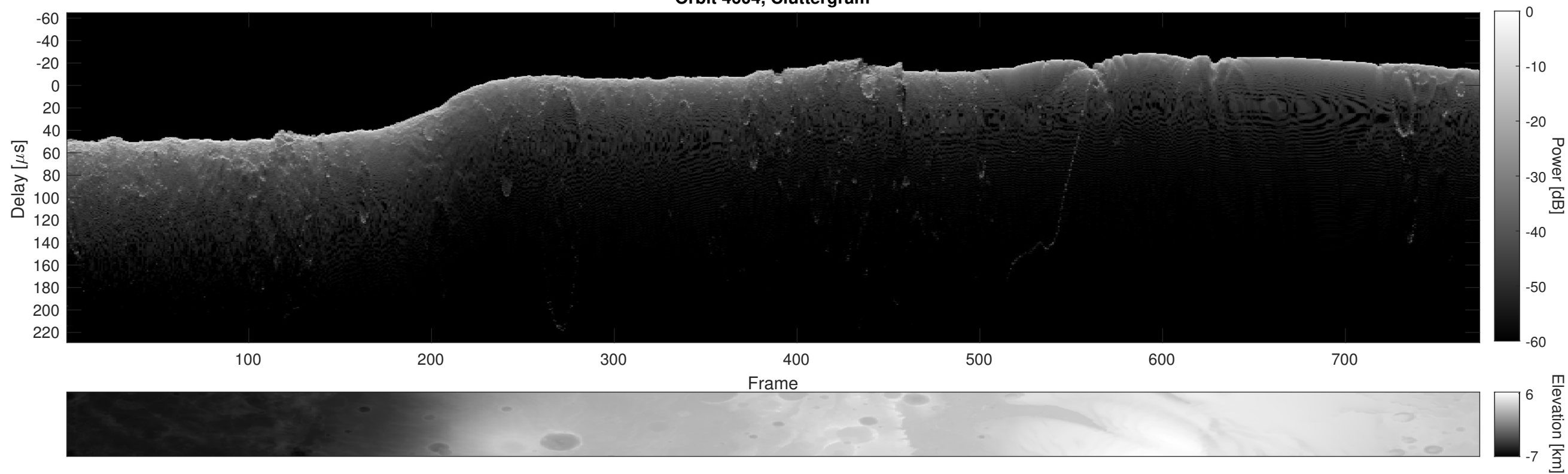
Orbit 4604, Cluttergram
