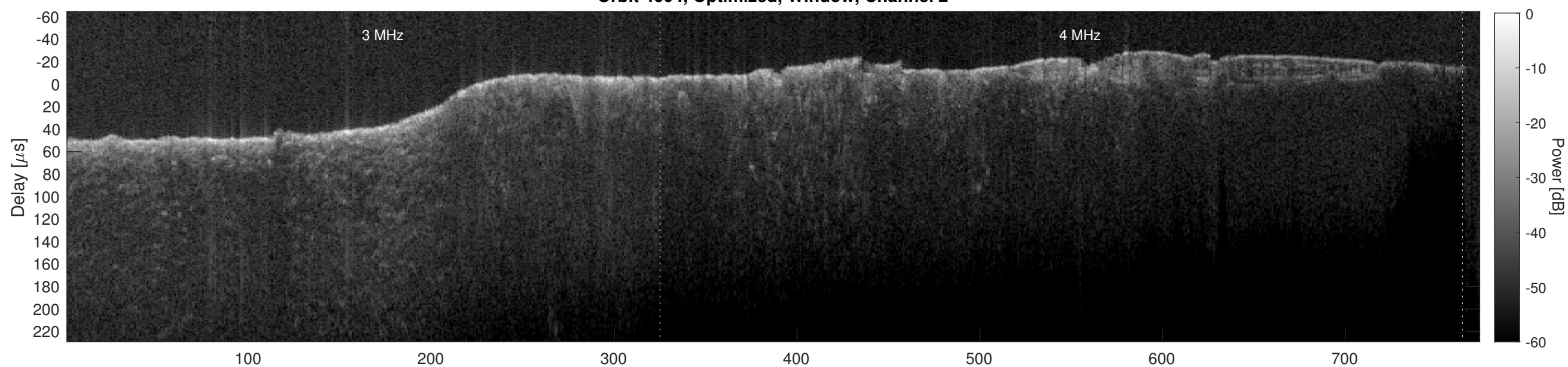
Orbit 4604, Cluttergram
