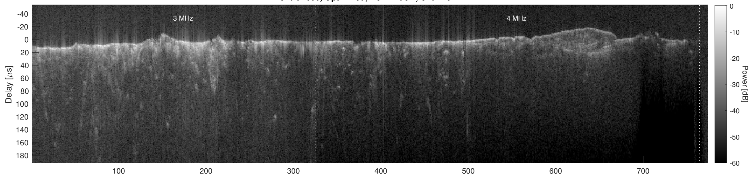
Orbit 4606, Cluttergram
