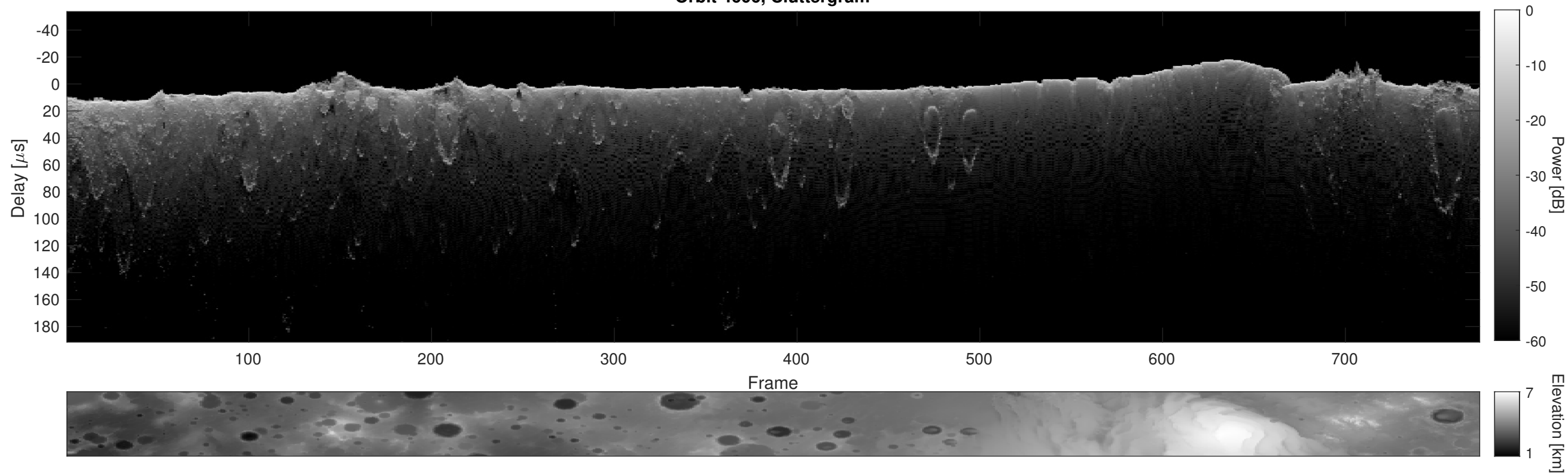
Orbit 4606, Cluttergram
