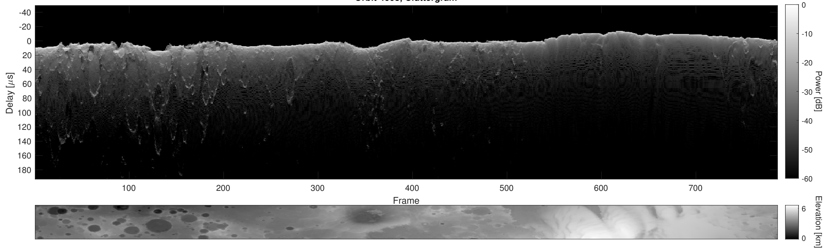
Orbit 4608, Cluttergram
