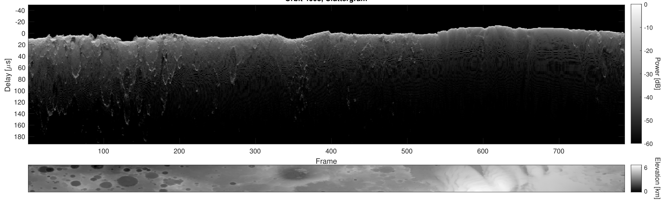
Orbit 4608, Cluttergram
