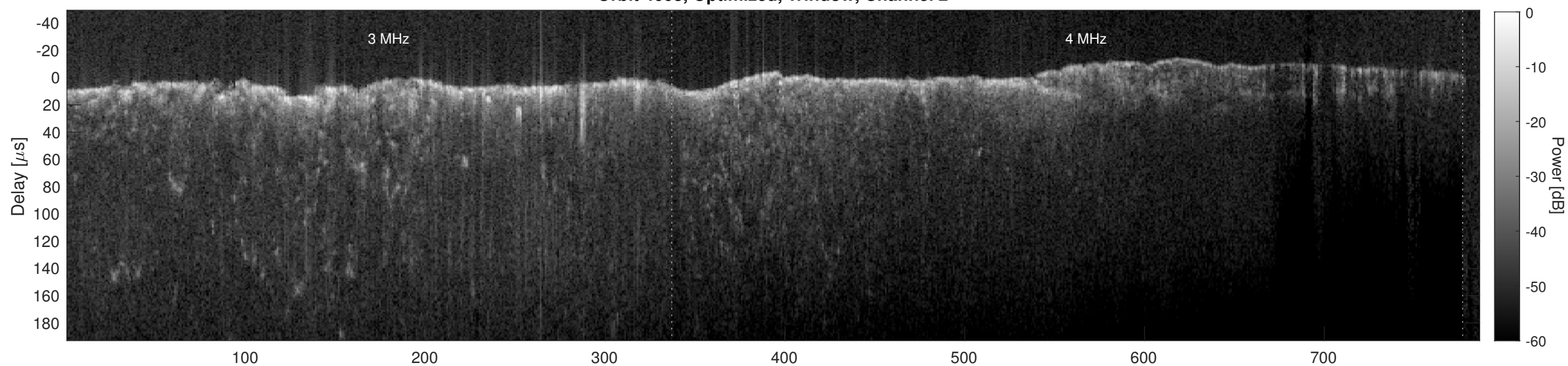
Orbit 4608, Cluttergram
