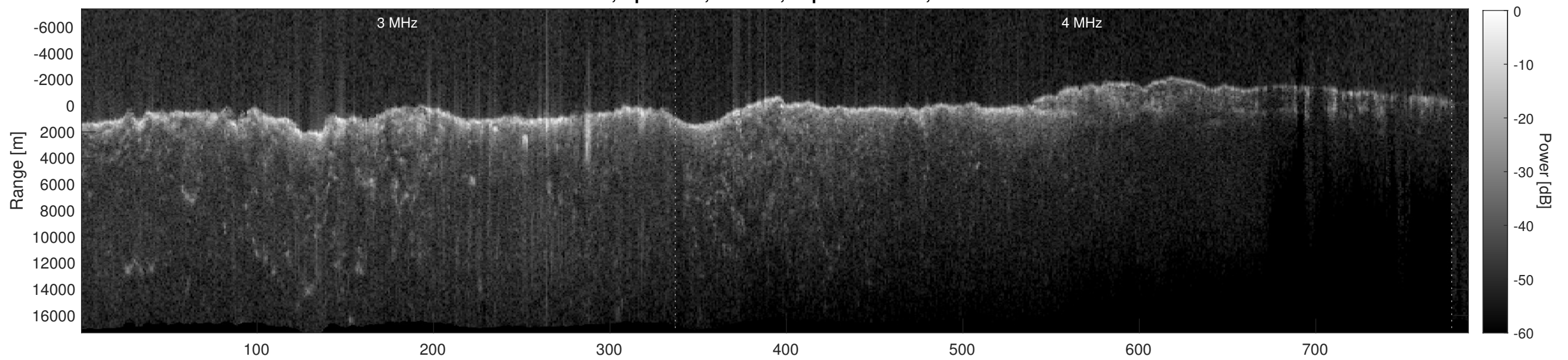
Orbit 4608, Depth-Corrected Cluttergram
