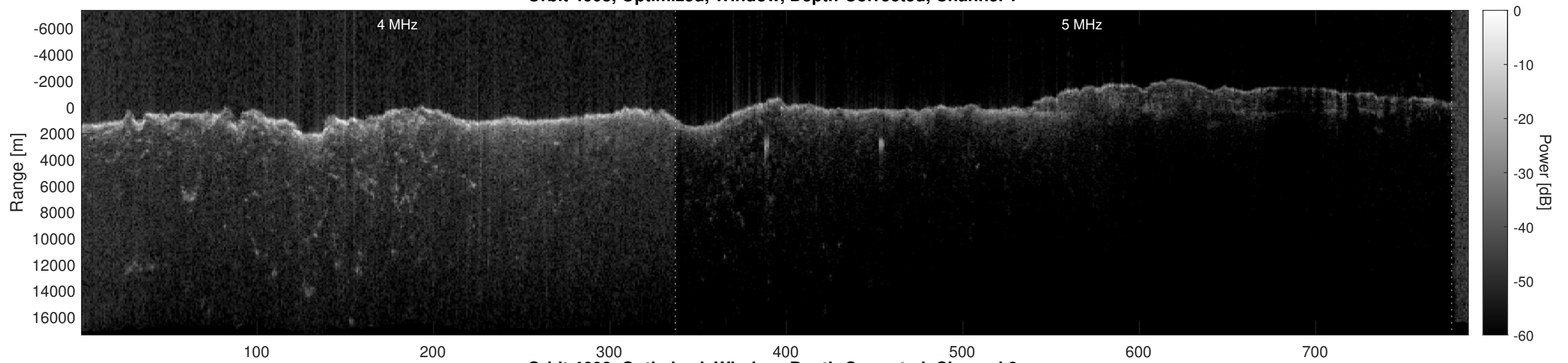
Orbit 4608, Optimized, Window, Depth-Corrected, Channel 2
