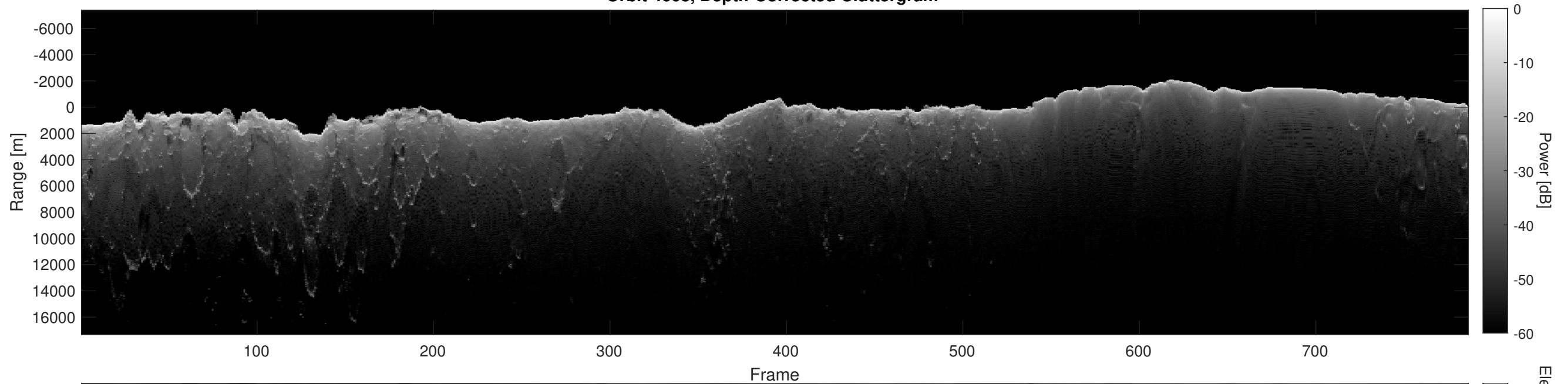
Orbit 4608, Depth-Corrected Cluttergram
