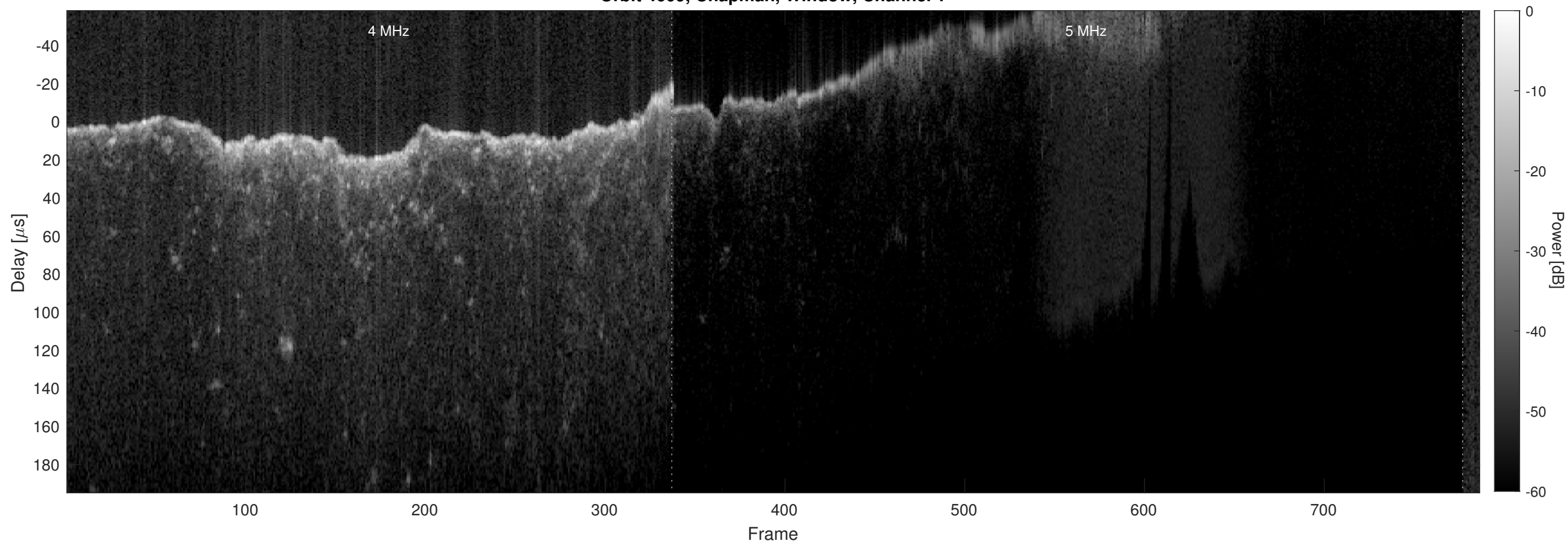
Orbit 4609, Chapman, Window, Channel 2
