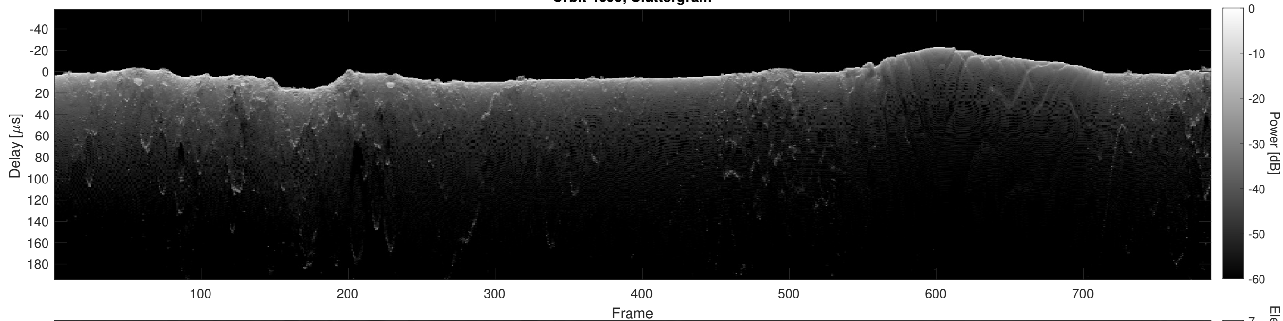
Orbit 4609, Cluttergram
