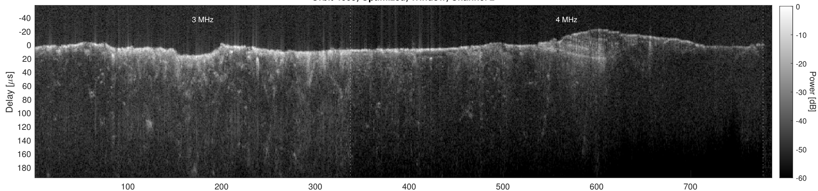
Orbit 4609, Cluttergram
