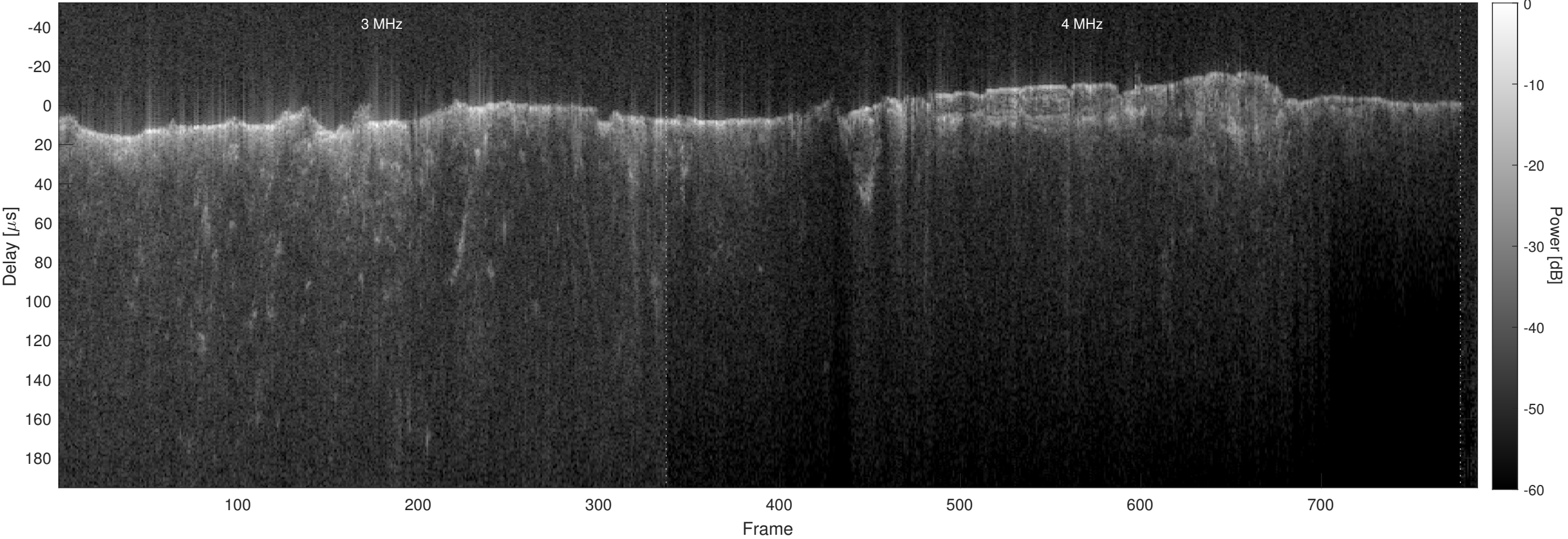
Orbit 4610, Optimized, No Window, Channel 2
