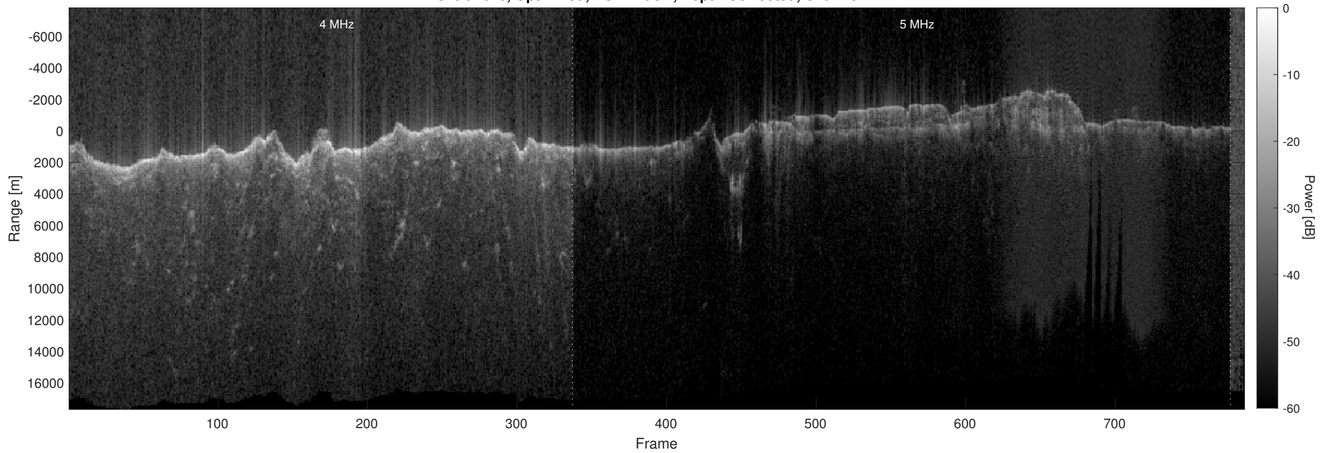
Orbit 4610, Optimized, No Window, Depth-Corrected, Channel 2
