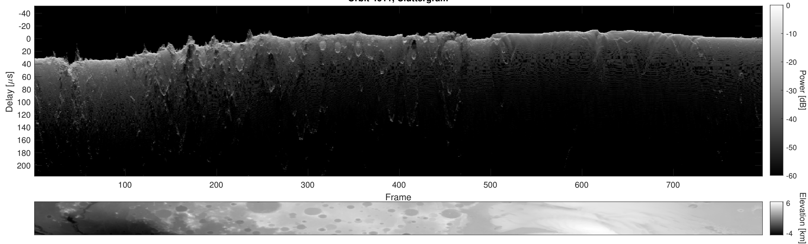
Orbit 4611, Cluttergram
