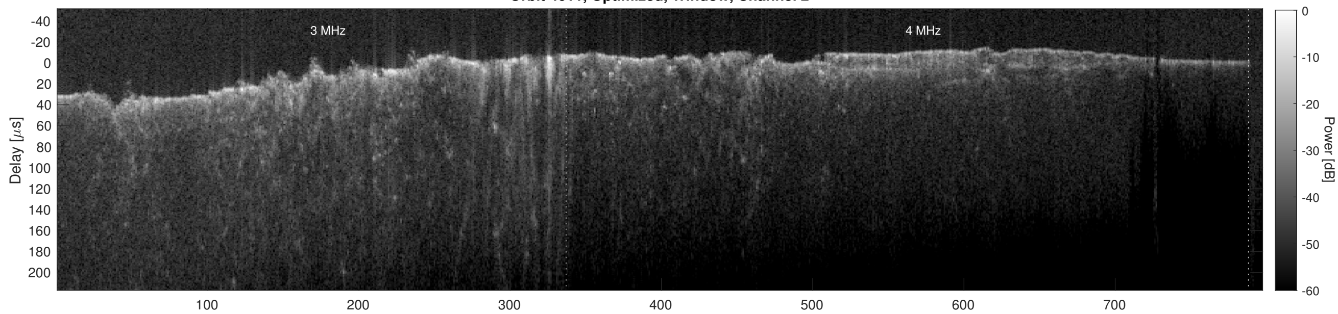
Orbit 4611, Cluttergram
