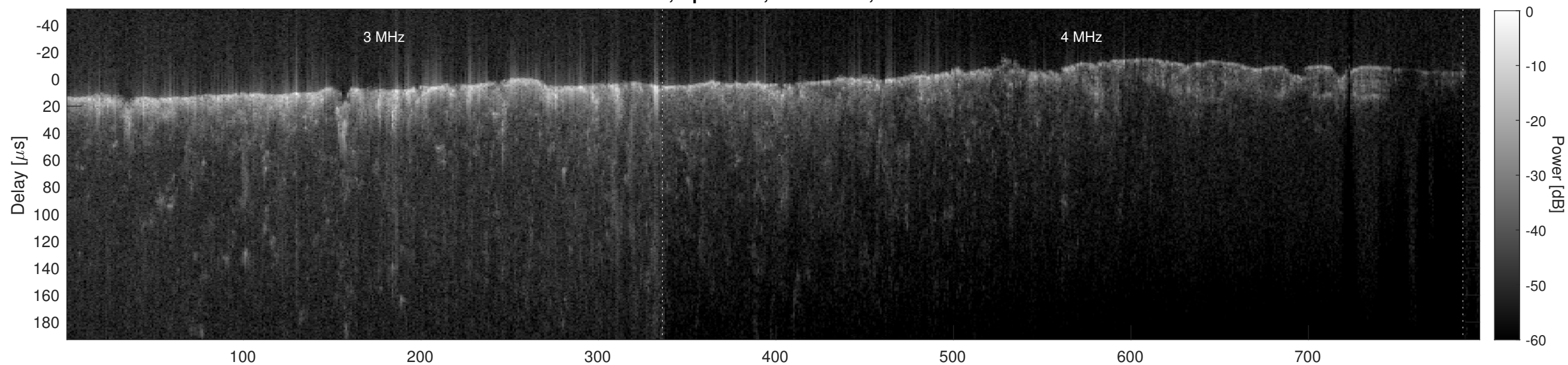
Orbit 4612, Cluttergram
