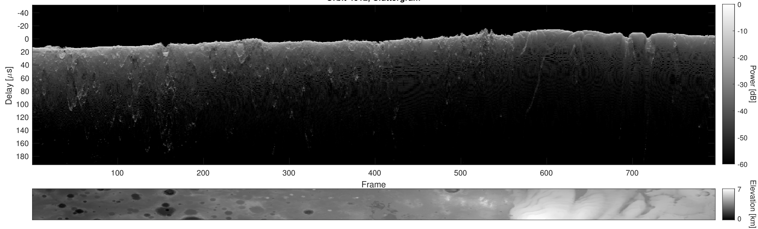
Orbit 4612, Cluttergram
