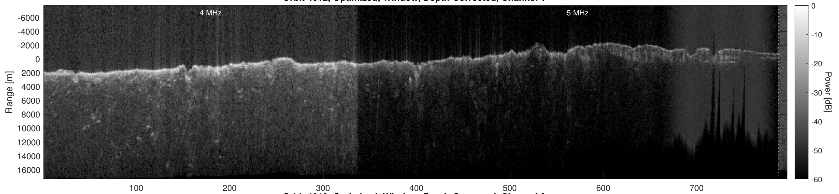
Orbit 4612, Optimized, Window, Depth-Corrected, Channel 2
