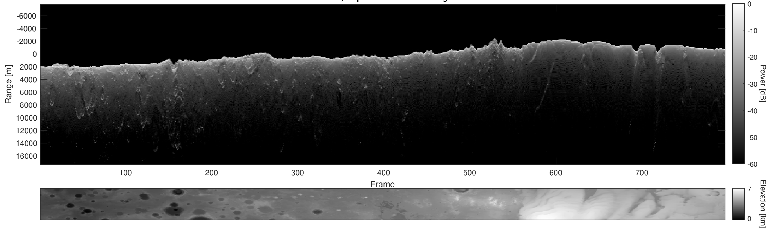
Orbit 4612, Depth-Corrected Cluttergram
