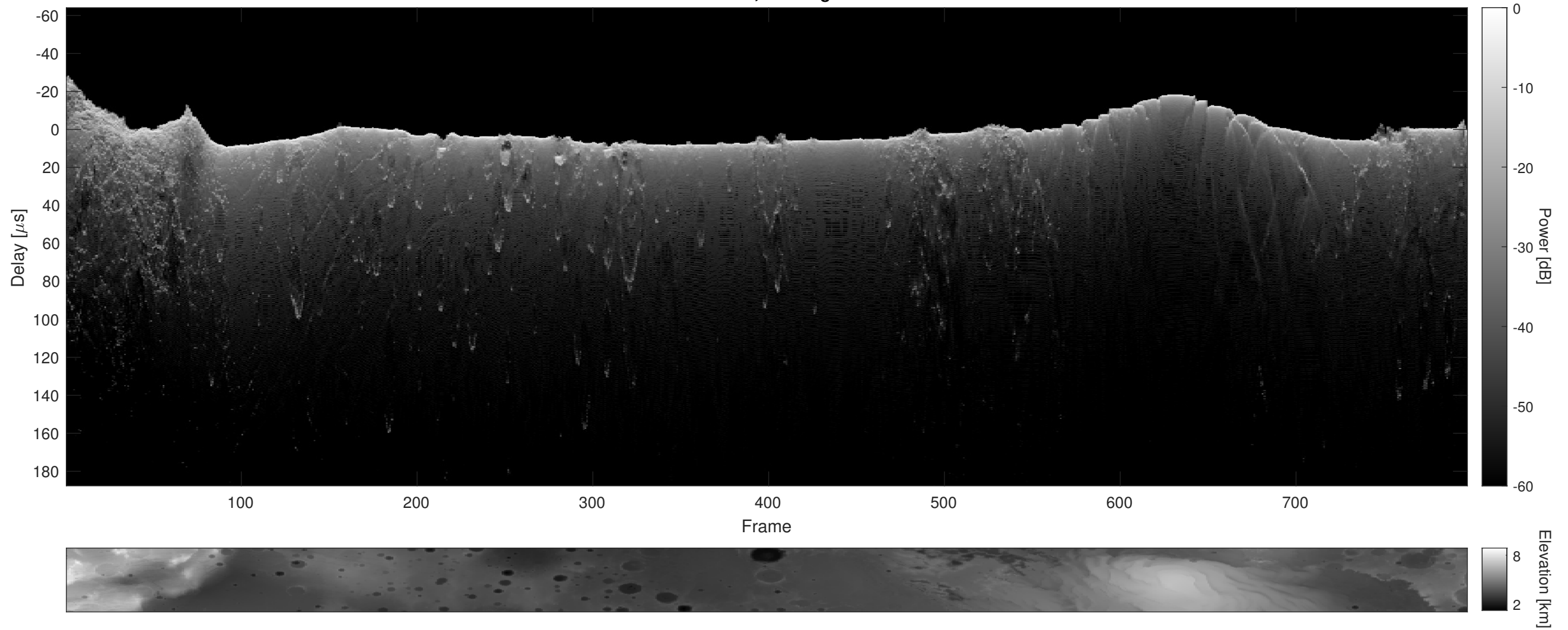
Orbit 4613, Cluttergram
