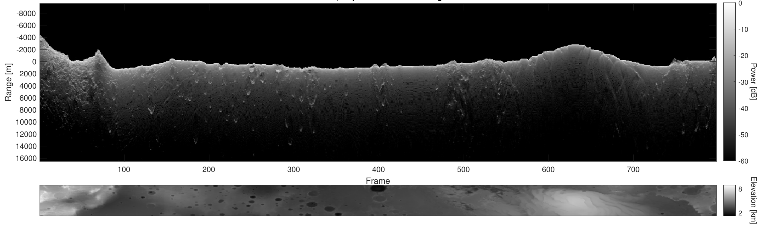
Orbit 4613, Depth-Corrected Cluttergram
