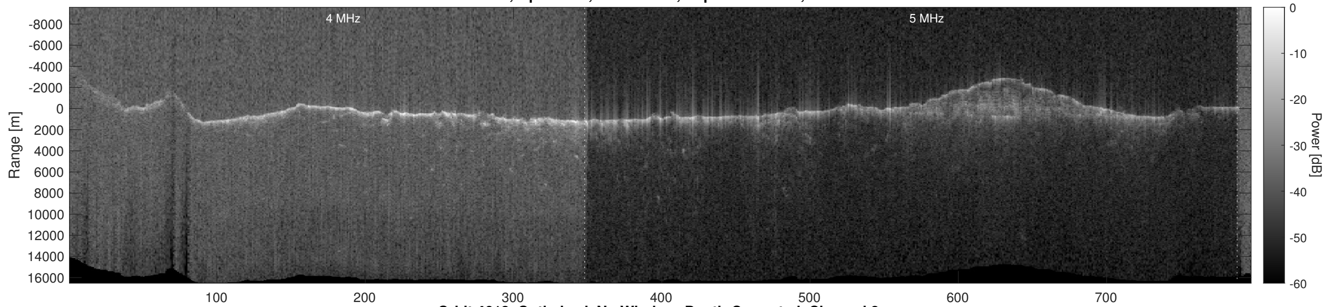
Orbit 4613, Optimized, No Window, Depth-Corrected, Channel 2
