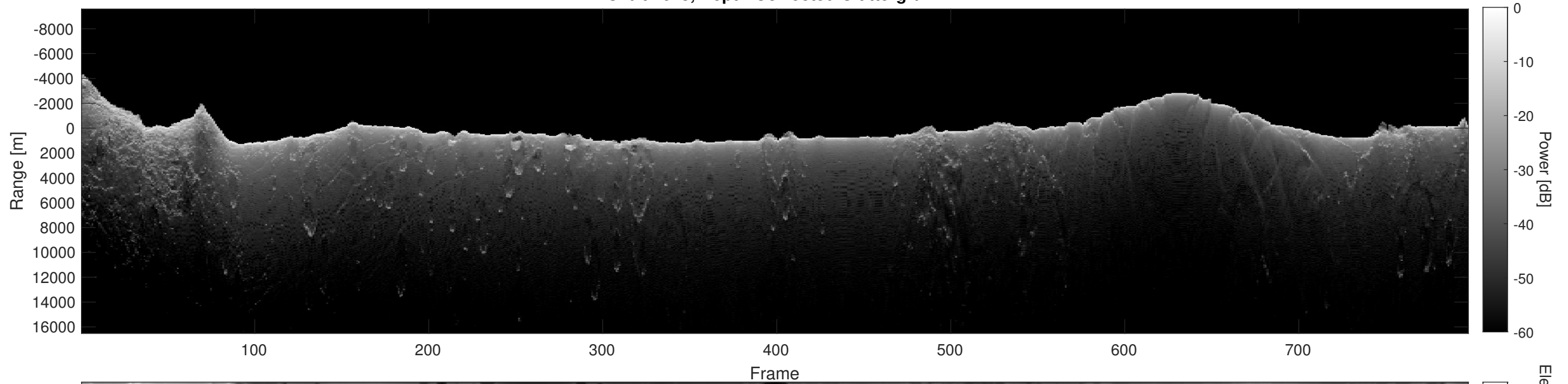
Orbit 4613, Depth-Corrected Cluttergram
