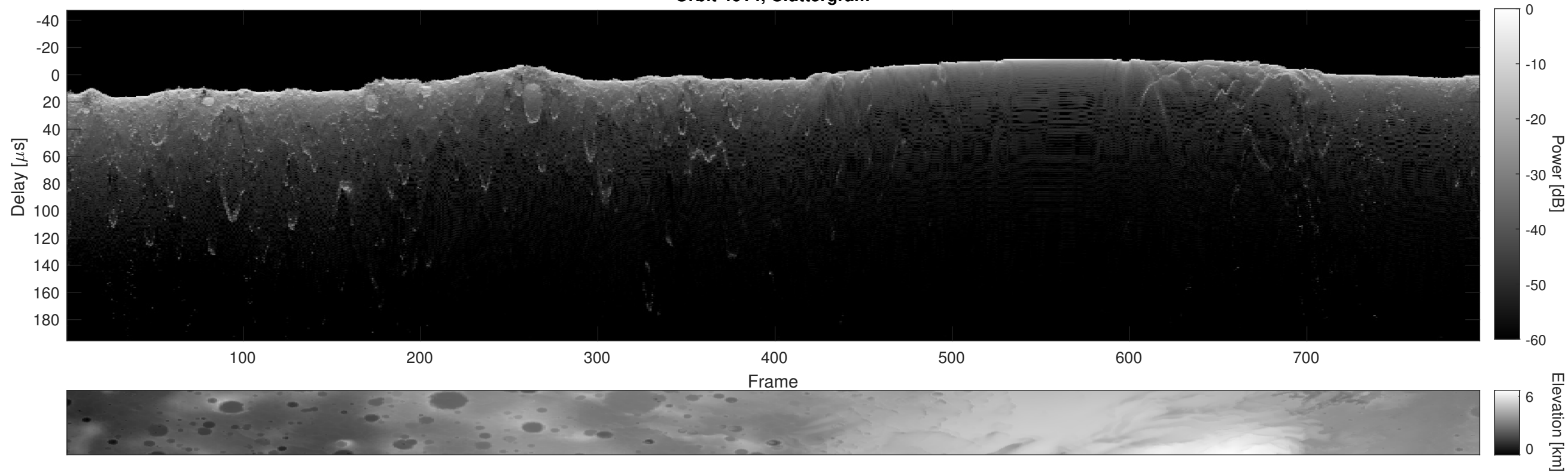
Orbit 4614, Cluttergram
