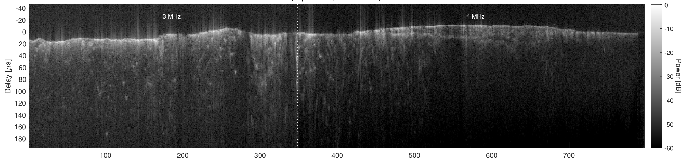
Orbit 4614, Cluttergram
