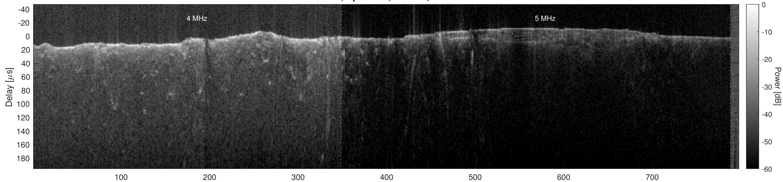
Orbit 4614, Optimized, Window, Channel 2
