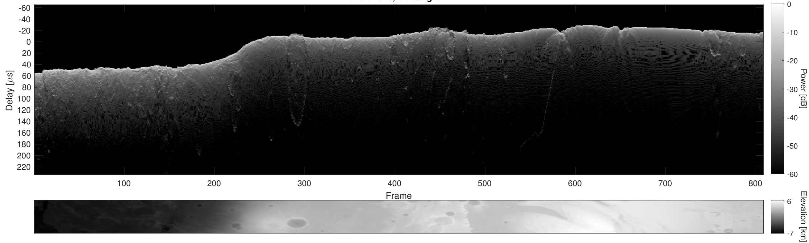
Orbit 4615, Cluttergram
