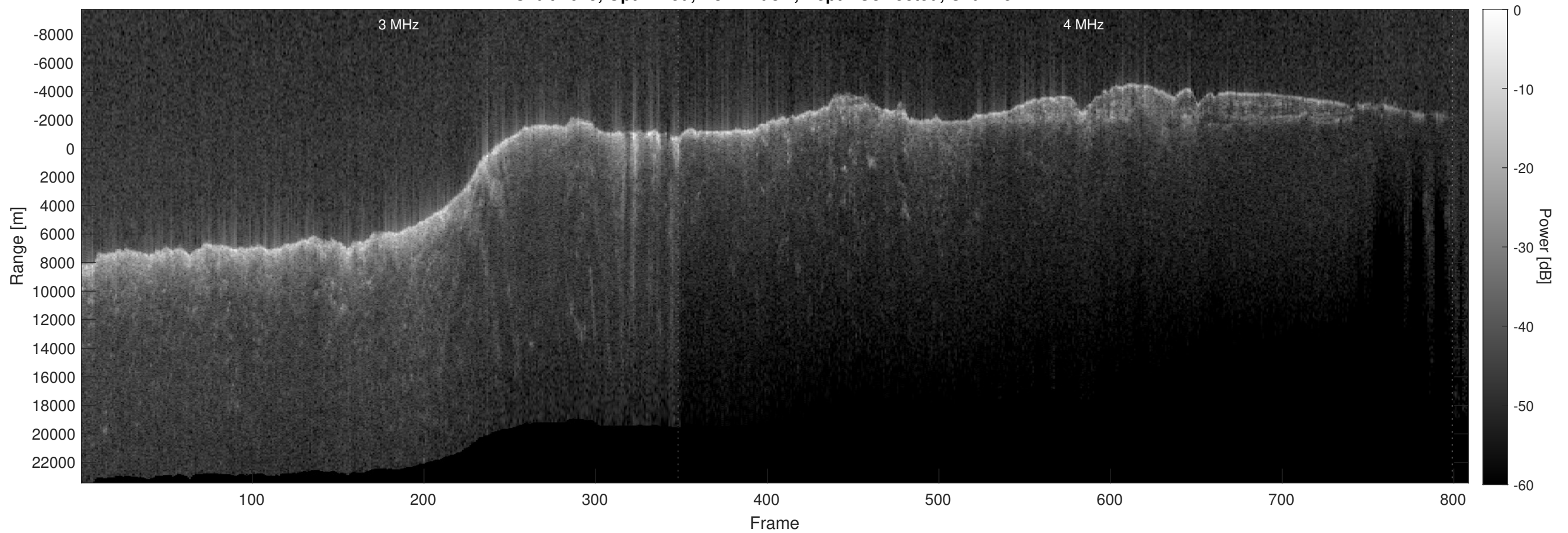
Orbit 4615, Optimized, No Window, Depth-Corrected, Channel 2
