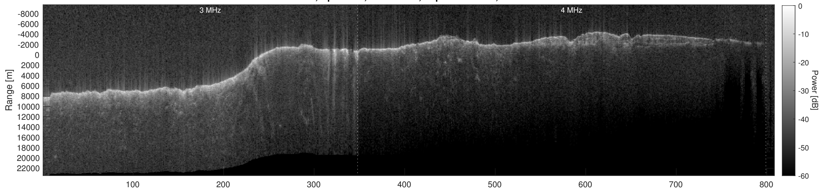
Orbit 4615, Depth-Corrected Cluttergram
