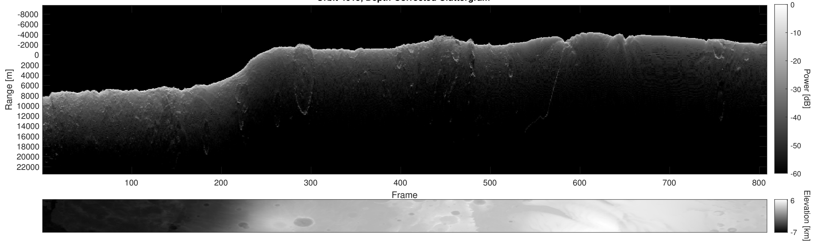
Orbit 4615, Depth-Corrected Cluttergram
