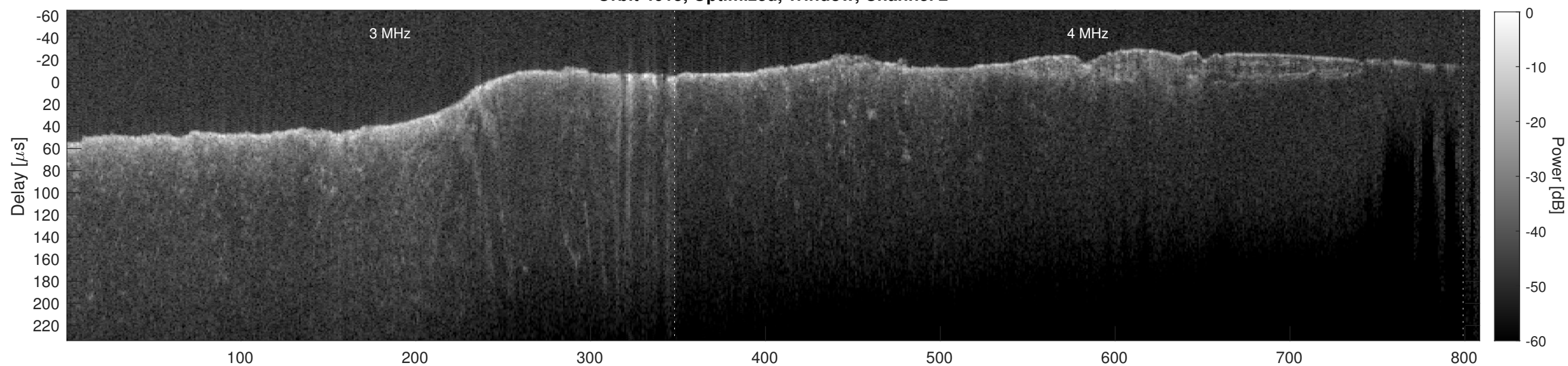
Orbit 4615, Cluttergram
