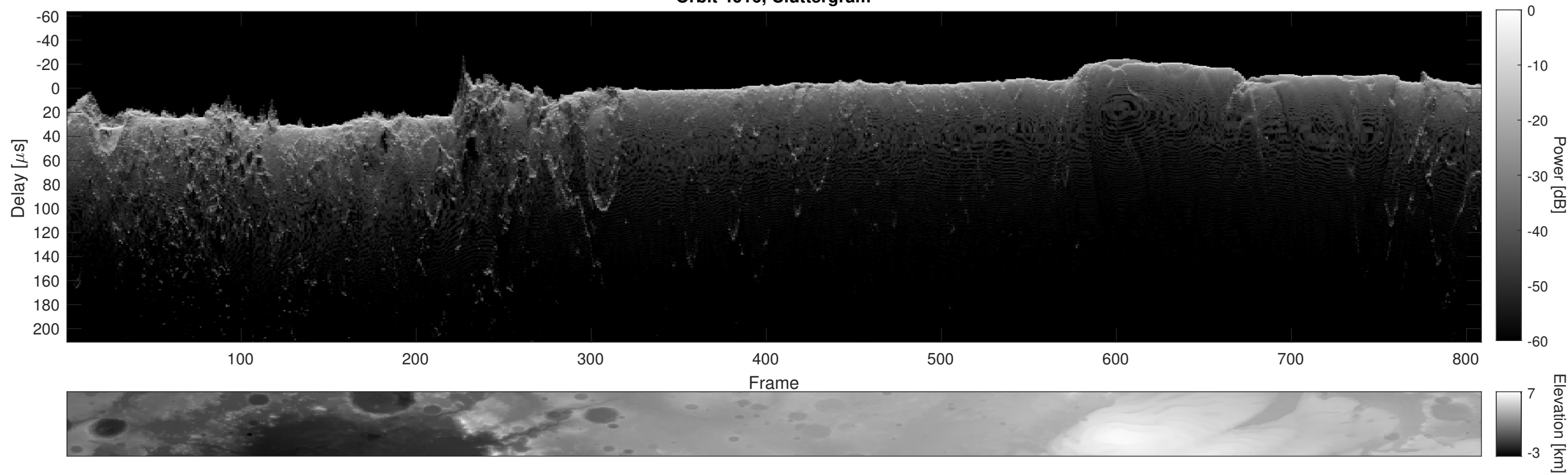
Orbit 4616, Cluttergram
