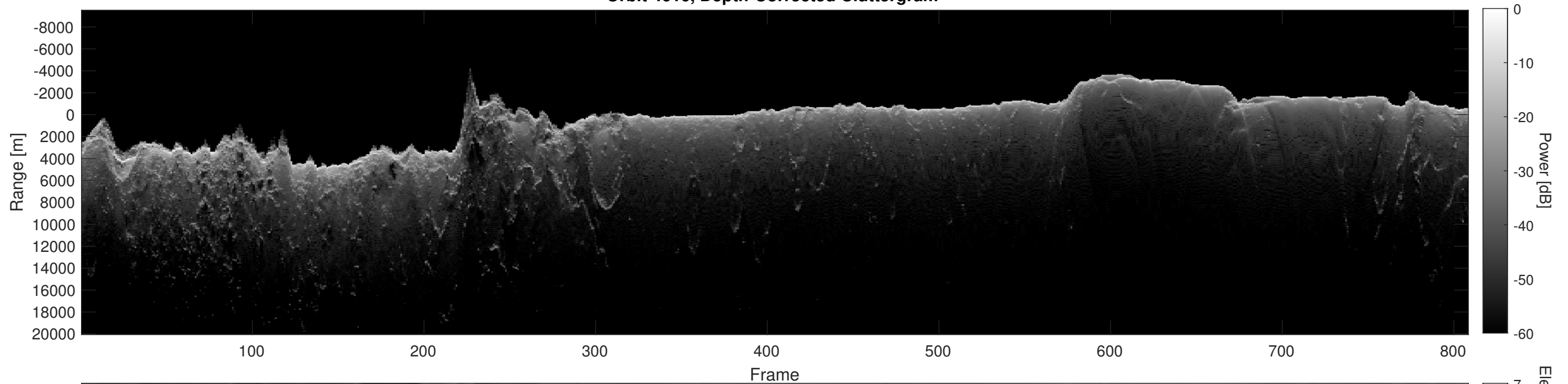
Orbit 4616, Depth-Corrected Cluttergram
