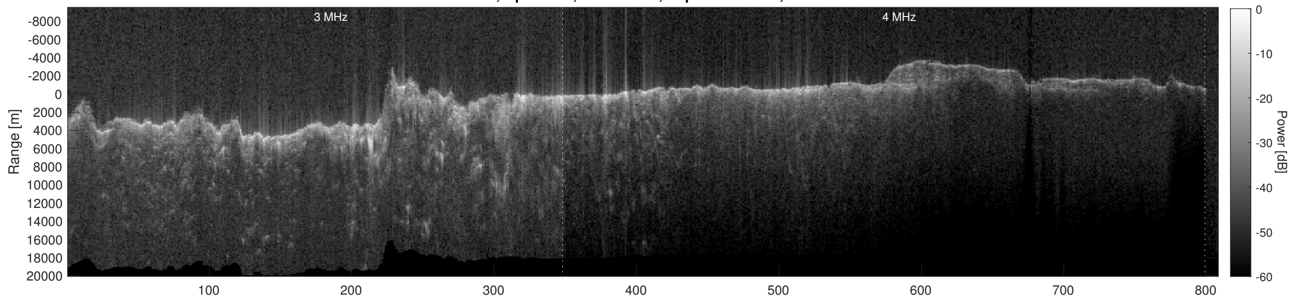
Orbit 4616, Depth-Corrected Cluttergram
