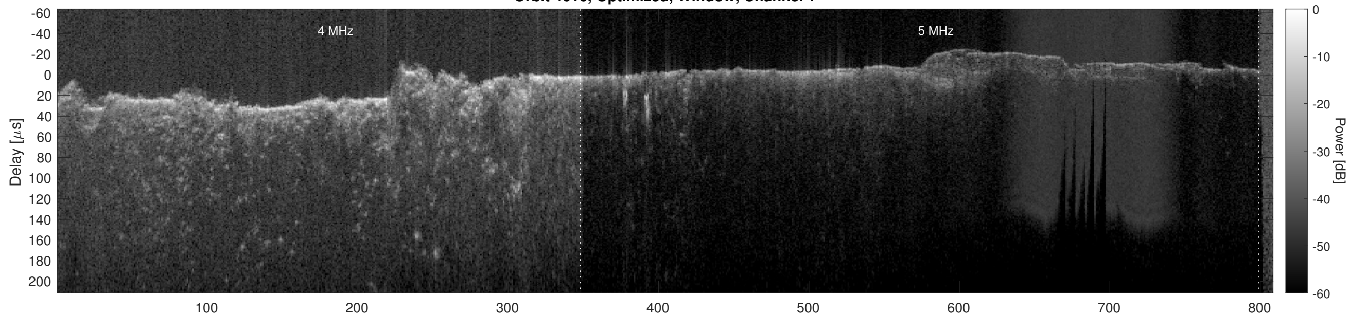
Orbit 4616, Optimized, Window, Channel 2
