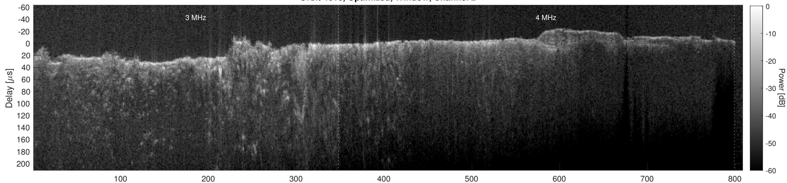
Orbit 4616, Cluttergram
