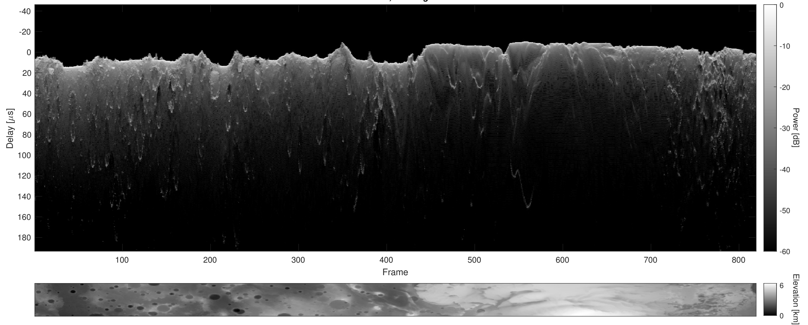
Orbit 4618, Cluttergram
